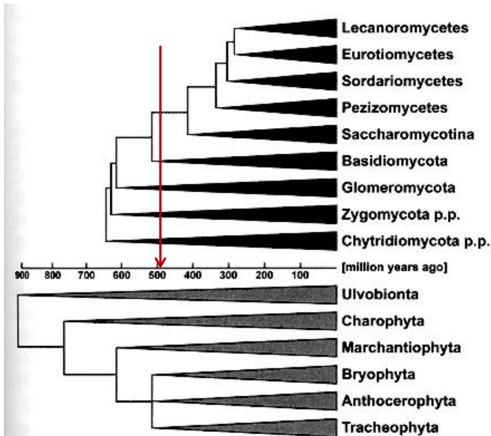
FIG. 2. The recalibrated fungal tree of life compared to the evolution of green plants, based on our most conservative estimates (TABLE IV). Green plant phylogeny and dating combined and simplified from various sources (Wang et al 1999; Heckman et al 2001; Hedges et al 2004; Yoon et al 2004, 2008; Steencamp et al 2006; Berbee and Taylor 2007; Moreira et al 2007; Zimmer et al 2007).
