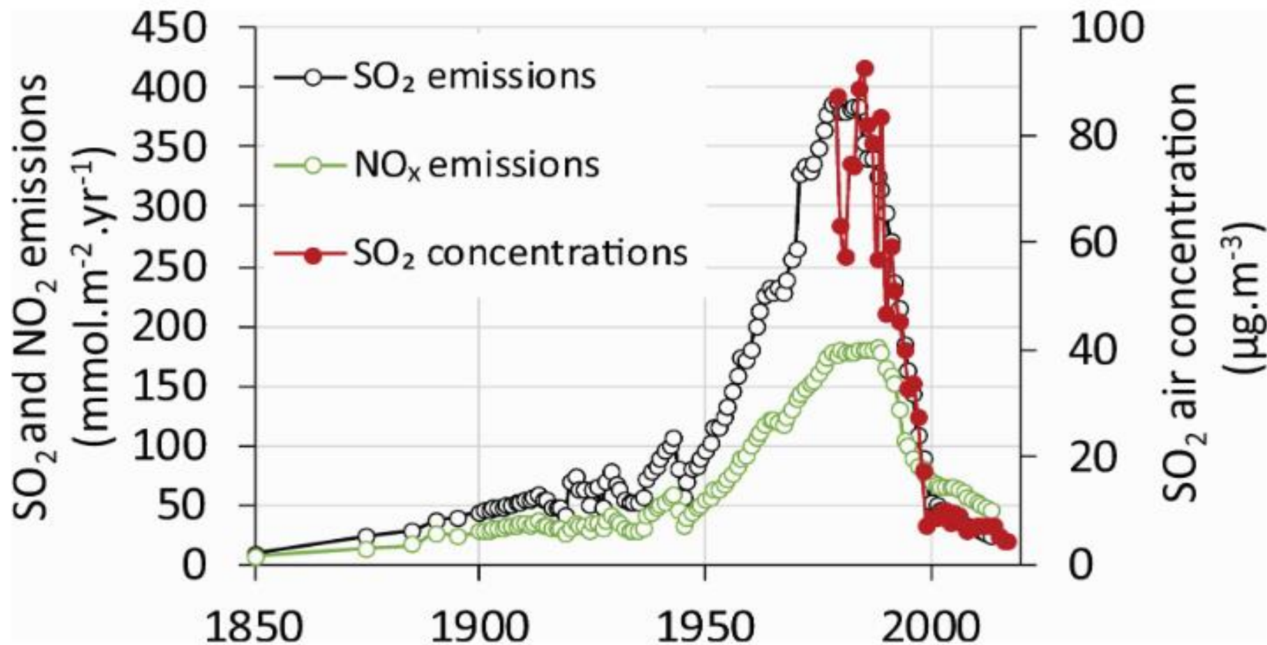
Fig 3. SO 2 emissions (Czech Republic) between 1850–2017 and ambient annual SO 2 concentrations measured at Cínovec (Zinwald) at the Czech/German border between 1979–2017.
