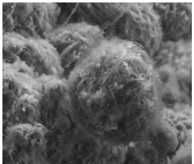
7/29/2009 Mag WD HV HFW Pressure Spot 50.0µm 4:08:40 PM 1200x 10.2 mm 20.0 kV 0.23 mm 230.0 Pa 3.5 Cladonia pleurota (T. -12°C)
