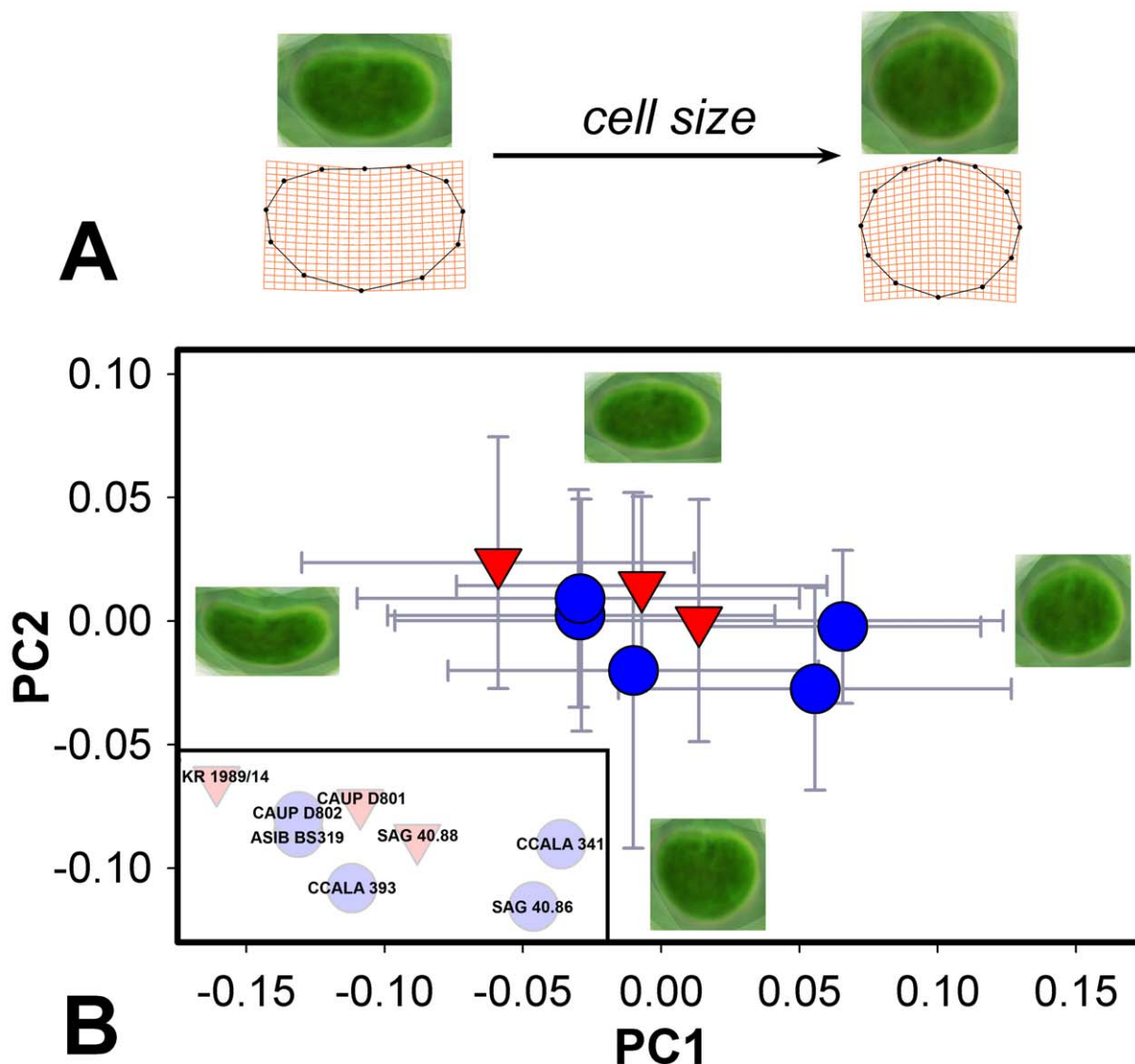
FIGURE 2: Morphometric characteristics of Neocystis strains. a) Visualisation of the multivariate regression model illustrating the relation of the shape and size of cells in the entire investigated dataset. b) The PCA ordination plot based on geometric morphometric data illustrating mean positions of individual strains and their standard deviations on PC1 (spanning 65.9% of the variation) and PC2 (23.2%). The theoretical cell shapes of marginal morphospace positions were reconstructed from the landmark coordinates of the original data.
