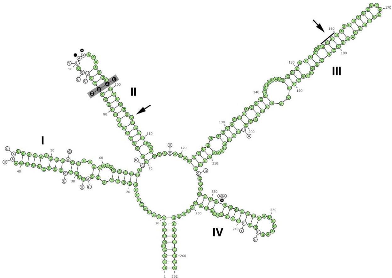
FIGURE 1: Comparison of the ITS2 sequences and predicted secondary structures of Neocystis brevis and Neocystis mucosa . Base numbering is indicated every 10 bases, and the four helices are numbered with Roman numerals. The structure shown corresponds to N. brevis ; positions conserved in N. mucosa are portrayed in green, bases substituted in N. mucosa are shown by the structure and connected to the respective position by a short line, insertions and deletions are indicated with plus and minus symbols, respectively. The base pair marked in a grey box is a compensatory base change (CBC). The highly conserved U–U mismatch in the helix II and UGGU motif in the helix III (Schultz et al. 2005) are marked by arrows.
