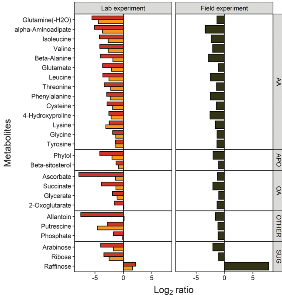
Fig. 5. Metabolites showing either a positive or negative differential accumulation between pre-akinetes and young cells (FDR adjusted t -test, P -value <0.01 , fold change >2 ) in both the field (right) and laboratory samples (left) are shown. \text{Log}_2 ratios of laboratory-grown stationary phase cells versus young cells (orange bars) and pre-akinetes versus young cells (red bars), and field-collected pre-akinetes versus young cells (black bars) are shown.
